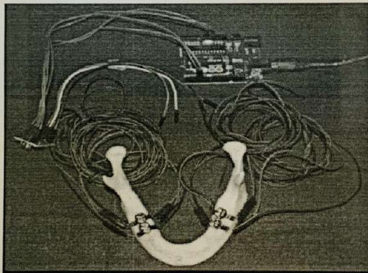
Electric circuit connected for strain testing
