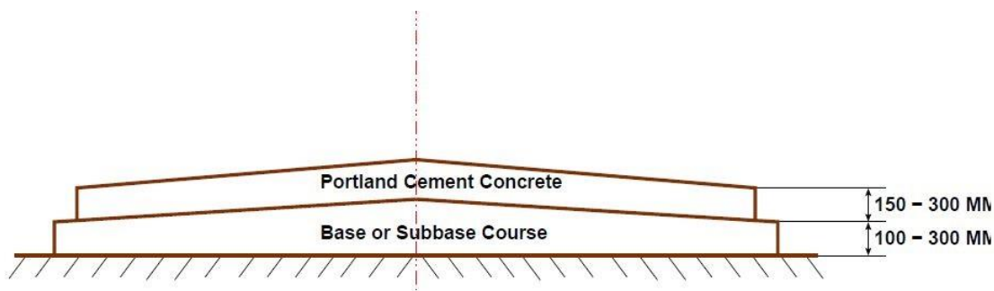
Typical Cross section of Rigid pavement
