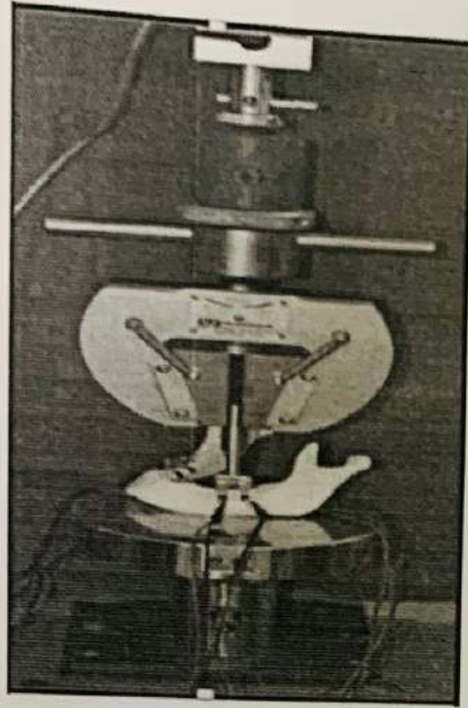
Load application using Universal testing machine
