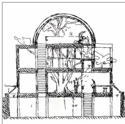
Sectional Sketch of Sangath Doshi's office at Ahmedabad, Gujarat
